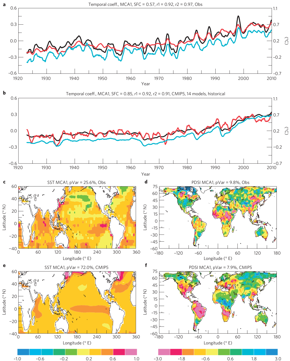
Figure 4 | Temporal and spatial patterns of the MCA1 mode for SST and sc+PDSI pm from observations and models. a–f , The blue line (right-side ordinate) is the global mean surface temperature from observations 31 in a and global mean surface air temperature from the models in b , which is the temporal coefficient of the MCA1 for the model SST (black) and sc_PDSI pm (red). The correlation between the black (red) lines in a and b is 0.85 (0.86) and the regression coefficient (with the observation as the predictor) between the SST (sc_PDSI pm ) anomalies represented by the MCA1 mode for the observation and models is 0.9119 (0.9566). The product of the temporal ( a,b ) and corresponding spatial ( c–f ) coefficients is the SST and PDSI anomaly represented by the MCA mode, with red areas experiencing warming (for SST) and drying (for PDSI) and blue areas for cooling and wetting.
