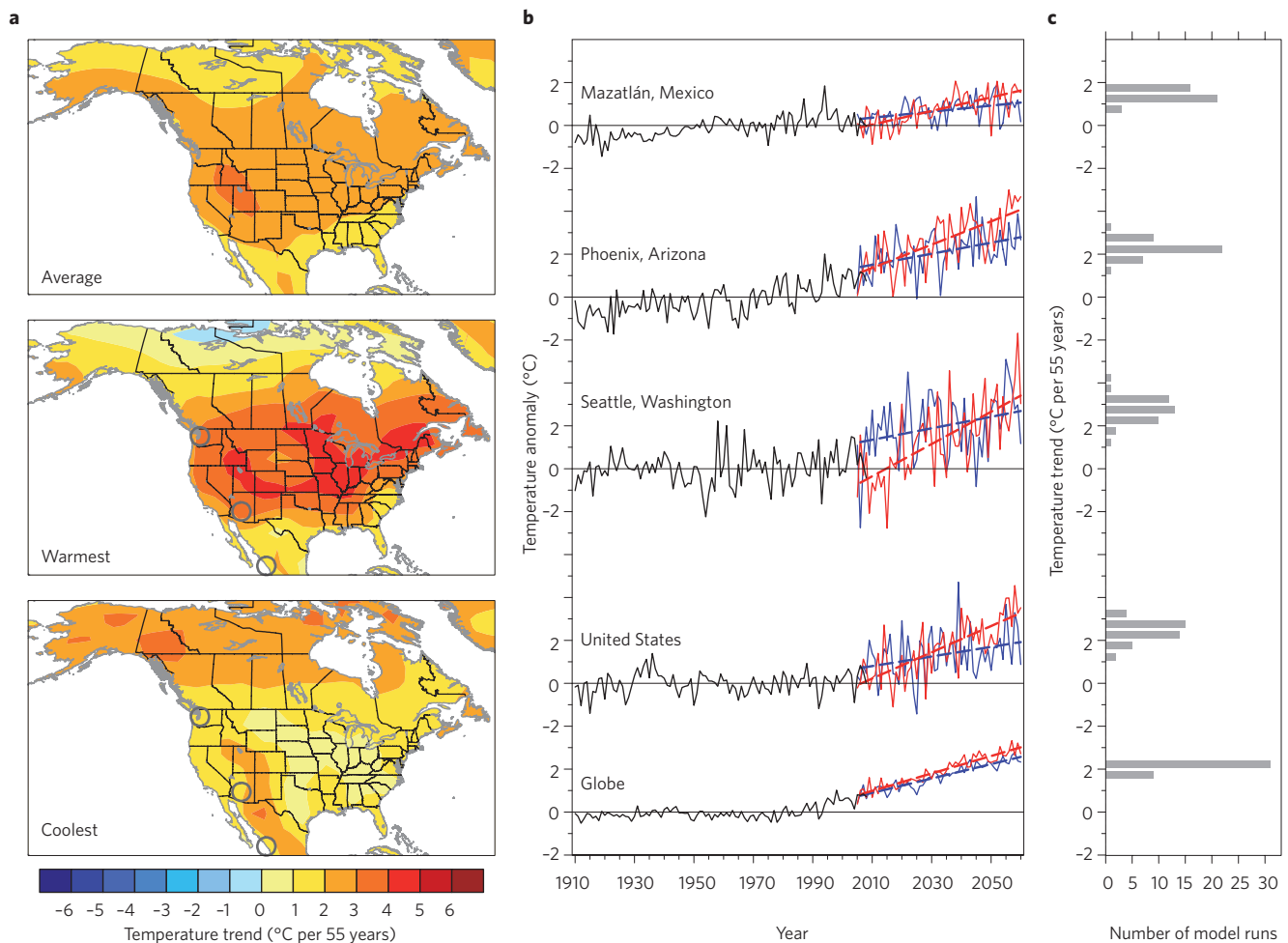
Figure 2 | Range of future climate outcomes. As in Fig. 1 but for June–July–August.
