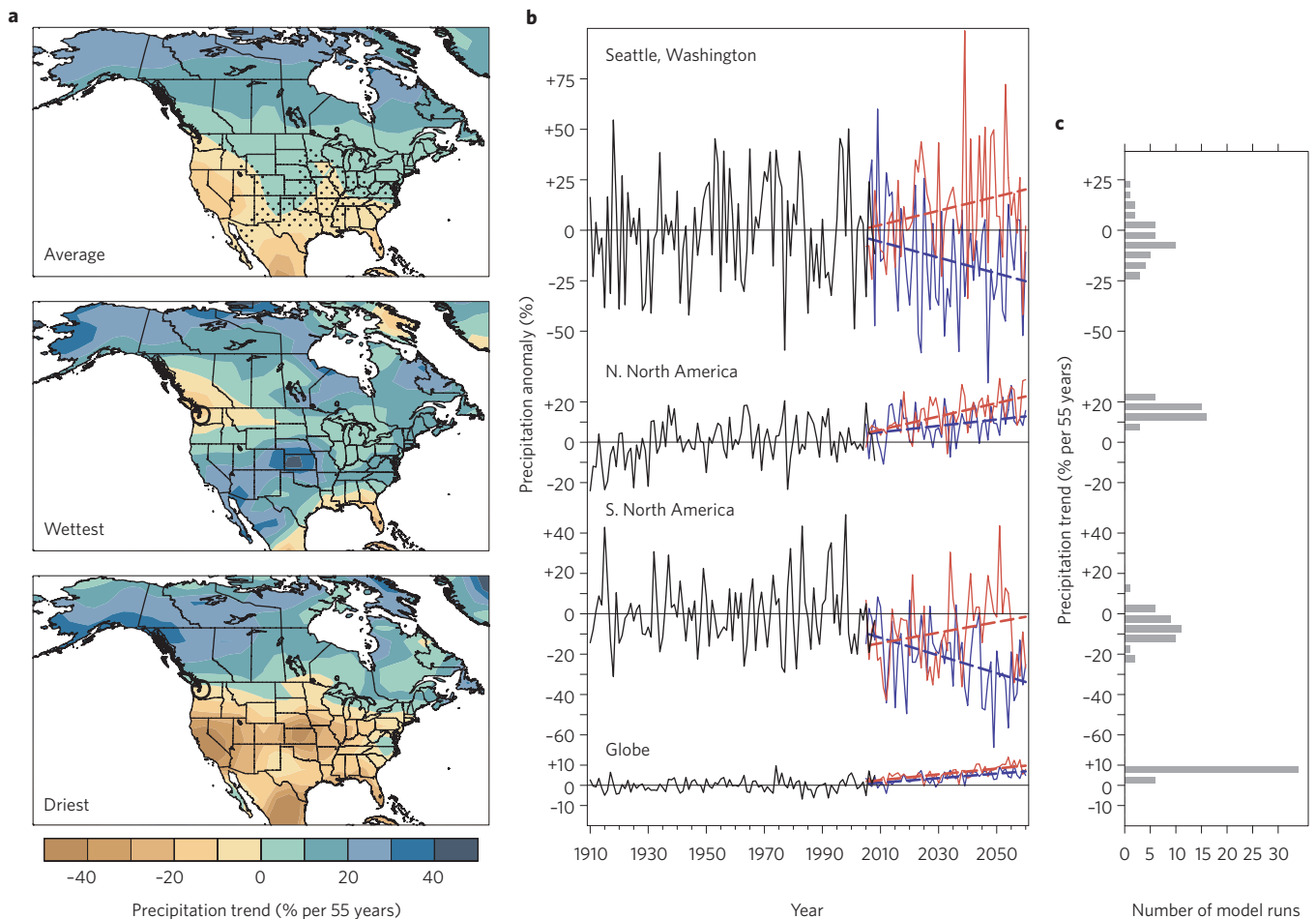
Figure 3 | Range of future climate outcomes. a , As in Fig. 1 but for December–January–February (DJF) precipitation trends, expressed as a percentage of the model’s ensemble-mean climatology for 2005–2060. Top panel shows the average of the 40 model runs, with stippling where the values are not statistically significantly different from zero at the 5% confidence level. The middle and bottom panels are based on the model runs with the wettest and driest trends for the southern half of North America (south of 42° N), respectively. b , DJF precipitation anomaly time series, expressed as a percentage of the observed mean during 1910–2008 minus 100%. Northern and southern North American regions refer to averages north of 50° N and south of 42° N, respectively. c , Distribution of projected DJF precipitation trends (2005–2060) across the 40 ensemble members at the locations shown in panel b .
